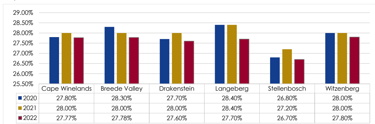
Graph 4: Learner-Teacher Ratio
