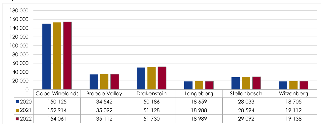
Graph 3: Learner Enrolment
