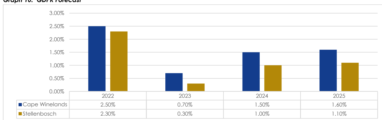
Graph 10: GDP Forecast
