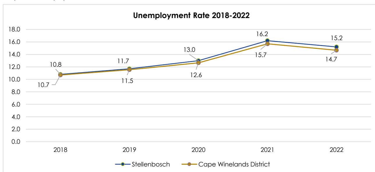
Graph 12: Unemployment Rate
